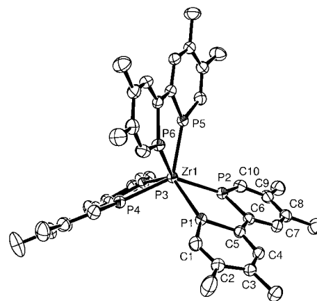
Figure 1. Structure of 4 in the crystal (50 % probability ellipsoids; hydrogen atoms omitted for clarity). Selected bond lengths [Å] and angles [ ^\circ ] of one biphosphinine unit: P1–Zr1 2.5441(8), P2–Zr1 2.563(1), P3–Zr1 2.551(1), P4–Zr1 2.5248(8), P5–Zr1 2.5486(8), P6–Zr1 2.532(1), P1–C1 1.753(3), C1–C2 1.362(4), C2–C3 1.428(5), C3–C4 1.368(4), C4–C5 1.414(4), C5–P1 1.779(3), C5–C6 1.434(4), C6–P2 1.779(3), P2–C10 1.752(3), C10–C9 1.380(5), C9–C8 1.429(5), C8–C7 1.370(5), C7–C6 1.422(4); P1–Zr–P2 69.91(3), C5–P1–C1 100.4(2).
