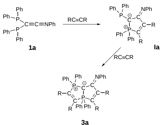
Scheme 2. Two [2+3] cycloaddition reactions of 1a with dimethyl acetylenedicarboxylate provide 3a . R = CO 2 Me.
